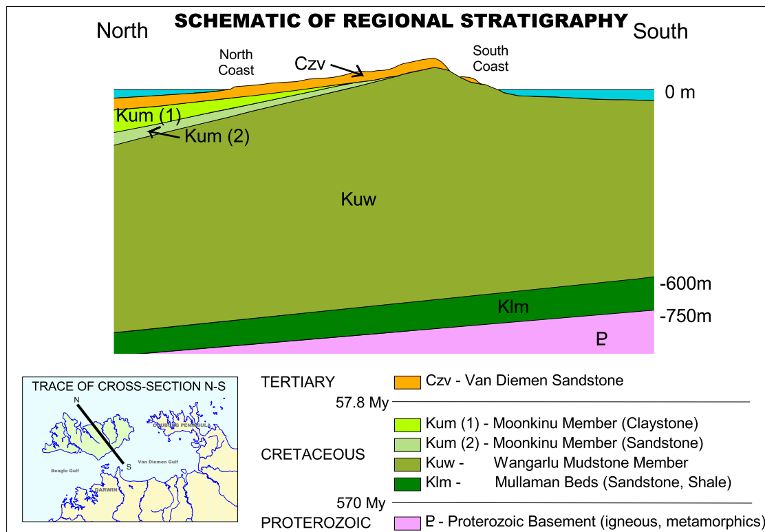
Figure 4 Regional Stratigraphy
