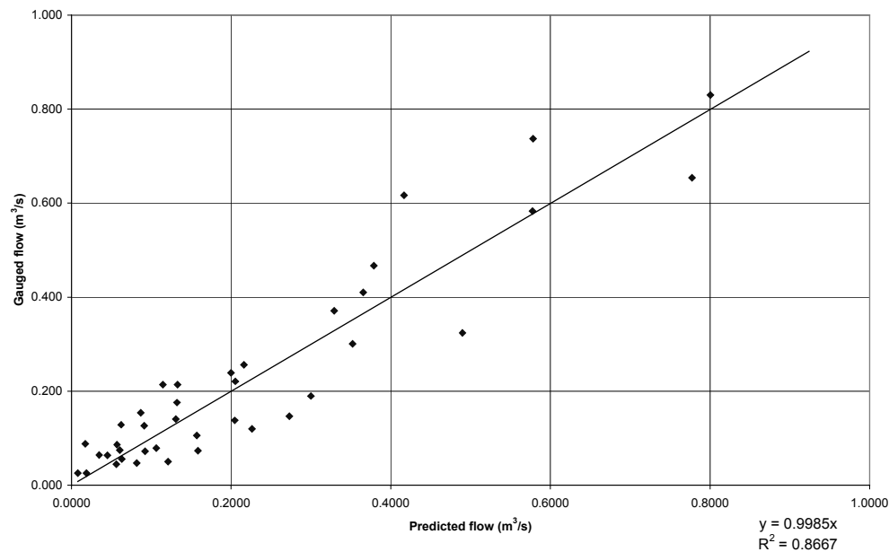
Figure 4.8. Relationship between predicted and actual gauged spring flow at G8160235, Takamprimili River at Dam Site, 1966 – 1985.
